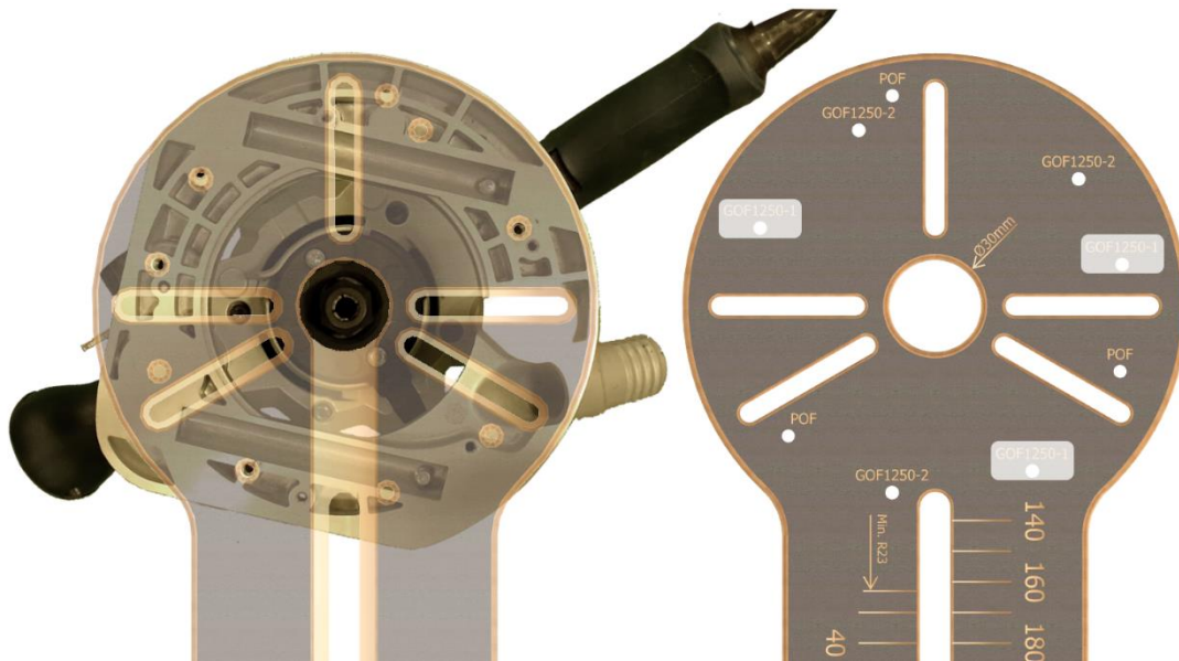
Figure 7- Mounting holes for Bosch GOF 1250-1
